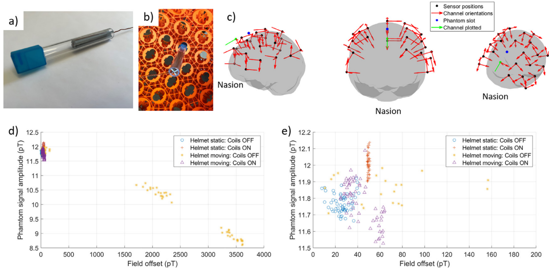
Fig. 5. Dry current dipole phantom and sensor gain experiments. (a) Photograph of the dry-type current dipole phantom used in these experiments. The phantom coil is an isosceles triangle wound around a (grey) plastic former with base 5 mm and height 65 mm. An empty (blue) OPM casing is attached to a (clear) Perspex cylinder into which the phantom coil is glued. (b) Photograph of the phantom inside the OPM-MEG helmet. The empty OPM casing can be inserted into any slot in the helmet, the base of the coil is 30 mm beneath the inner surface of the helmet. (c) Each of the 23 triaxial OPMs (black dots) used in the experiment are shown around the template brain, which was used to design the helmet surface. Red arrows indicate the three channel orientations for each OPM. The slot into which the phantom was inserted is shown in blue. (d) Plot of the field amplitude measured on a single channel (indicated by the green dot and arrow in (c)) due to a 200 nA, 23 Hz phantom signal, Results are shown for four experimental cases. Note that during the experiment in which the helmet moved but the matrix coils were not active a large range of field offsets and phantom signal amplitudes are recorded due to sensor gain changes as the field experienced by the OPM moves away from zero. (e) Zoomed in plot of data for low field offsets (0 - 200 pT) to show consistency of measured source amplitude in the other three experiments.
