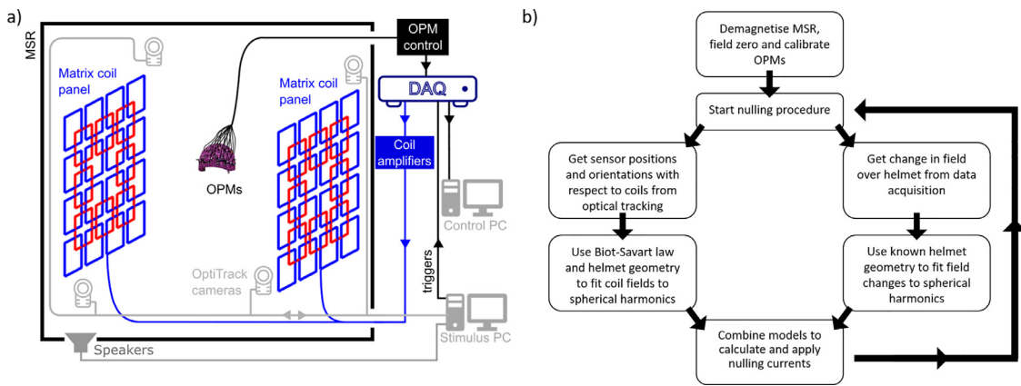
Fig. 2. System schematic and nulling procedure flowchart. (a) Overview of OPM-MEG system with matrix coils. The system is housed in a magnetically shielded room. Coil panels are placed either side of a participant wearing a helmet that contains OPMs. A control PC is used to read incoming data from the OPMs and optical tracking cameras then combine these data to calculate and apply nulling currents. A separate PC is used during MEG experiments to provide (in this case) auditory stimulation to a participant via a set of speakers. Trigger channels are used to synchronise the stimuli to the OPM recording. (b) Flowchart of continuous field nulling process.
