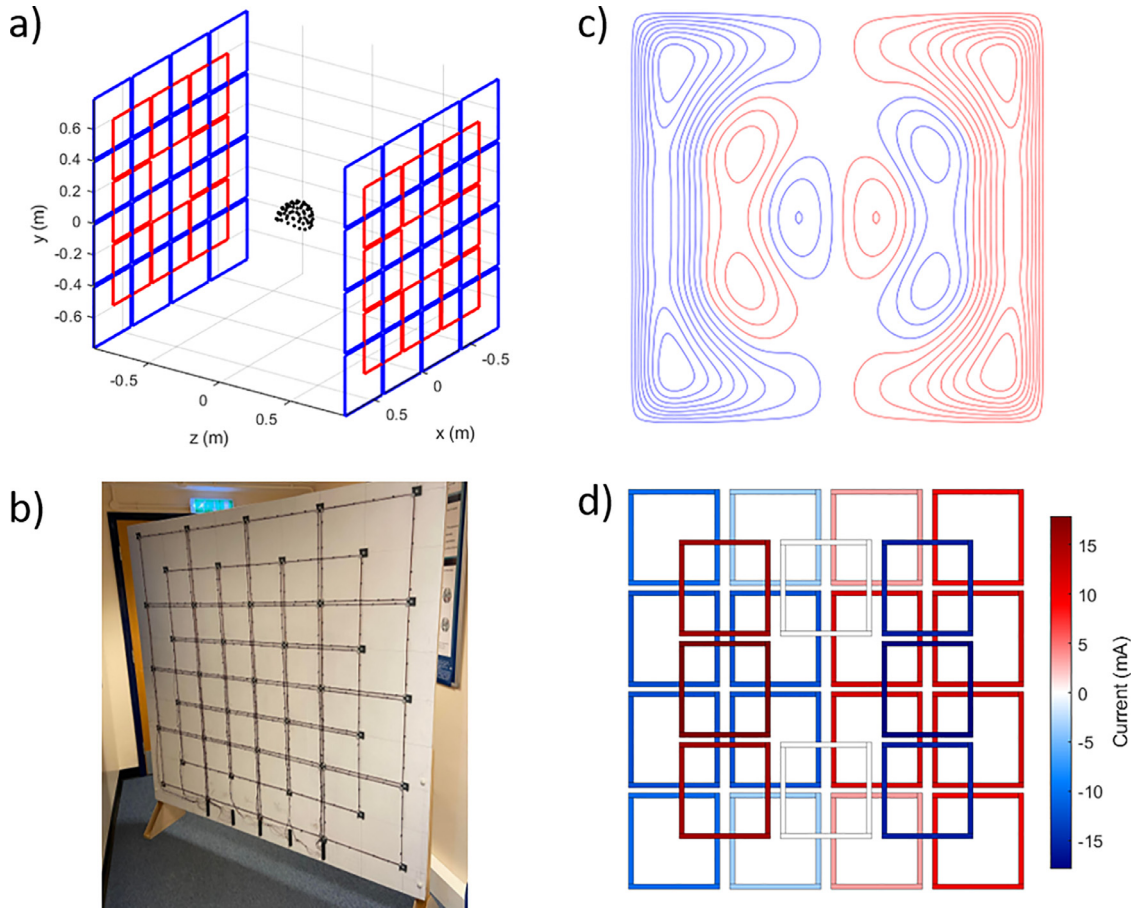
Fig. 1. The matrix coil active magnetic shielding system. (a) System is arranged in a bi-planar geometry and each plane contains 24 square coils arranged in an overlapping grid pattern. The blue and red colours highlight the 4 \times 4 grid of coils and the overlapping 3 \times 3 (excluding the central coil) set of coils. The black dots represent the positions of OPM sensors in a 3D printed helmet placed at the centre of the coils. (b) Photograph of a single plane of the constructed coil system. (c) The distributed windings of one plane of a bi-planar coil designed to generate a uniform magnetic field in the x-direction (see (a)) over a 40 \times 40 \times 40 \text{ cm}^3 volume at the centre of the two planes with deviation <5\% from the target magnetic field. Such designs have been used in previous OPM-MEG experiments. Red and blue denote regions of opposing current flow. The second plane (not shown) features the same windings, but the current directions are reversed with respect to the first plane. (d) The currents applied to one plane of the matrix coil to generate the same field as the coil shown in (c), note the similarity between the two designs in terms of current distribution and direction of current flow. The current directions in the second plane are again reversed.
