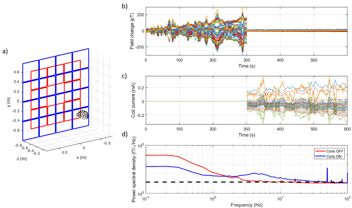
Fig. 3. Compensating magnetic field drifts on a fixed array of OPMs. (a) The position of the helmet containing 15 triaxial OPMs with respect to one plane of the matrix coils. The helmet is deliberately positioned off centre in the x , y and z directions to showcase the flexibility of the matrix coil system to generate the required compensation fields at multiple locations between the planes (helmet centre of mass (x,y,z) = (0.15, -0.24, 0.18) m). (b) Magnetic field drifts recorded by the OPMs over a period of 600 s. Each colour represent an individual channel. For the first 300 s the matrix coil system was not active, for the final 300 s the matrix coil compensated changes in the uniform field and field gradients over the helmet. (c) The current applied to each of the 48 coils throughout the experiment. Each colour represents an individual coil current. Note the similarity between the profile of the field changes in the first half of the experiment and the current variations in the second half of the experiment. (d) The power spectral density of the data measured by the OPMs with the coils off (red) and with the coils on (blue). The low-frequency noise level is reduced by the matrix coil, but an increase in noise is seen at higher frequencies. The black dashed line indicates 15 \text{ fT}/\sqrt{\text{Hz}} , the noise floor of the OPMs used in the experiments.
