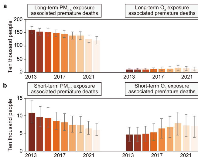
Fig. 7. Premature deaths associated with long-term and short-term exposure to \text{PM}_{2.5} and \text{O}_3 in China from 2013 to 2021. a. Trends in premature deaths associated with long-term air pollution exposure. b. Trends in premature deaths associated with short-term air pollution exposure. Data source: estimated in this study based on method in Xiao et al., 2022 [22].
