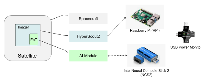
Fig. 3. Illustration of the emulation system hardware setup, featuring the Raspberry Pi as the HyperScout2 sensor emulator and the Intel Neural Compute Stick 2 (NCS2) as the AI module emulator.
