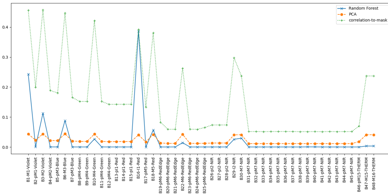
Fig. 2. Comparative visualization of band importance as determined by Pearson Correlation to the smoke mask (COR), Principal Component Analysis (PCA), and Random Forest (RF) methods in the context of band selection for AI onboard fire smoke detection. The three methods effectively identify the 11 original bands from VIIRS imagery but with different prioritization of bands by each method.
