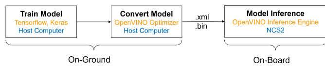
Fig. 5. A schematic representation of the AI model preparation process for onboard inference, detailing the steps of model training, model converting using OpenVINO optimizer, and model inference on the NCS2.
