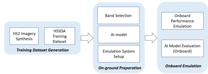
Fig. 1. overview of the pre-launch phase for AI onboard fire smoke detection. There are three main components of the workflow: (1) Training Dataset Generation, where HyperScout-2 (HS2) imagery is synthesized to create a pre-labeled training dataset covering a diverse range of fire smoke conditions; (2) On-Ground Preparation, which involves tasks such as band selection analysis, AI model preparation, and setting up and tuning the emulation system; (3) Onboard Emulation, depicting the emulation of onboard performance and the evaluation of the AI model in an onboard setting.
